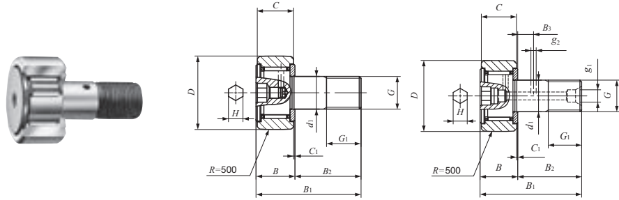
CF...BR 杆端直径 d_1 3~10mm CF...BUUR 杆端直径 d_1 12~30mm CF...BUU 杆端直径 d_1 12~30mm
