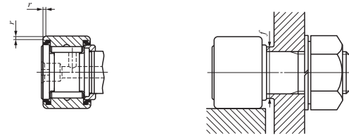
CRH...VUU
