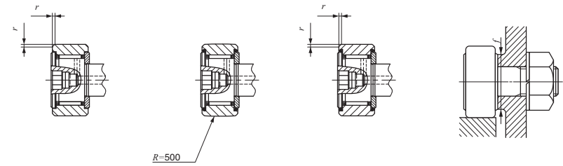
CF...B CF...BUUR CF...BUU
